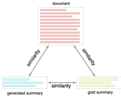
Figure 1: We enforce the similarities between the document, gold summary and model generated summary.
